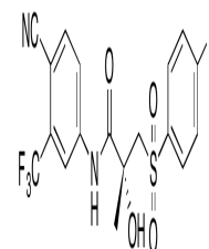
Chemical structure of R-Bicalutamide
