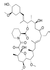
Chemical structure of Tacrolimus
