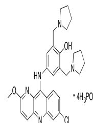
Chemical structure of Pyronaridine Tetra...
