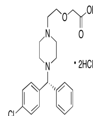
Chemical structure of Levocetirizine Dihydrochloride
