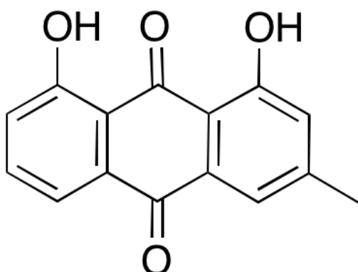
Chemical structure of Chrysophanol
