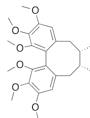
Chemical structure of R-(+)-Schisandrin
