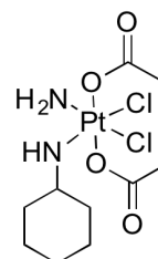
Chemical structure of Satraplatin
