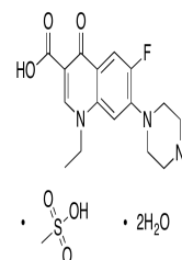
Chemical structure of Pefloxacin Methane...
