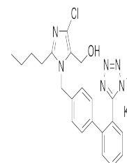
Chemical structure of Losartan Potassium
