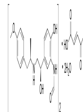
Chemical structure of Formoterol Fumarat...
