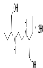
Chemical structure of Ethambutol Dihydro...
