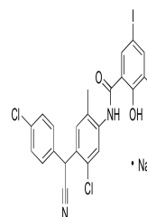
Chemical structure of Closantel Sodium
