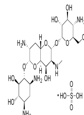
Chemical structure of Apramycin Sulfate
