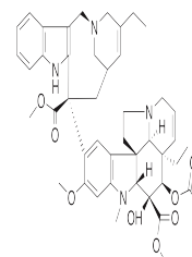
Chemical structure of Vinorelbine Base
