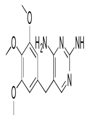
Chemical structure of Trimethoprim
