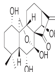
Chemical structure of Rubescensin A
