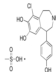
Chemical structure of Fenoldopam Mesylat...
