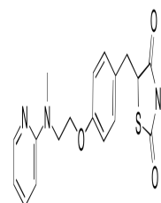
Chemical structure of Rosiglitazone
