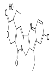
Chemical structure of 7-Ethyl-10-hydroxy...
