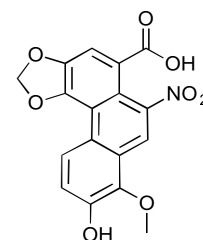
Chemical structure of 7-Hydroxyaristoloc...
