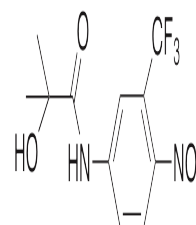
Chemical structure of 2-Hydroxyflutamide
