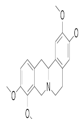
Chemical structure of D
