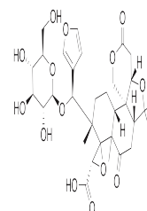
Chemical structure of Limonin Glucoside
