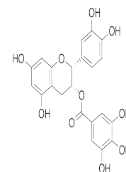
Chemical structure of (-)-Epicatechin gallate
