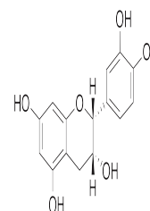
Chemical structure of (-)-Epicatechin
