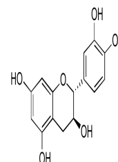
Chemical structure of (+)-Catechin
