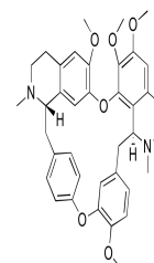
Chemical structure of S
