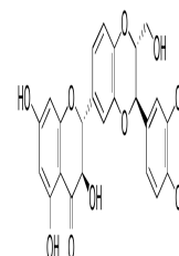
Chemical structure of Silybin
