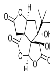
Chemical structure of (-)-Bilobalide
