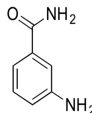
Chemical structure of 3-Aminobenzamide
