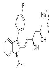
Chemical structure of Fluvastatin Sodium
