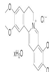
Chemical structure of Palmatine Chloride...
