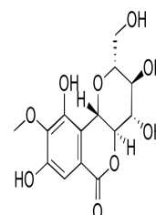
Chemical structure of Bergenin
