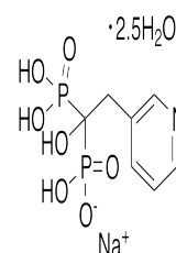
Chemical structure of Risedronate Sodium...
