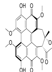
Chemical structure of Hypocrellin A
