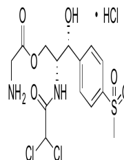
Chemical structure of Thiamphenicol Glyc...
