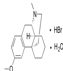
Chemical structure of Dextromethorphan H...
