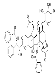
Chemical structure of Xylosyltaxol
