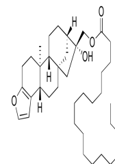
Chemical structure of Cafestol Stearate
