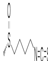
Chemical structure of S-Sulforaphane
