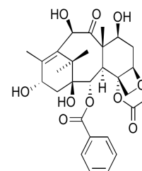
Chemical structure of 10-Deacetylbaccati...
