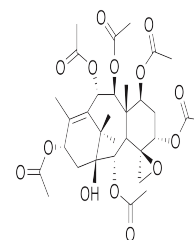
Chemical structure of 1-Hydroxybaccatin
