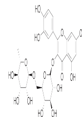
Chemical structure of Rutin Hydrate
