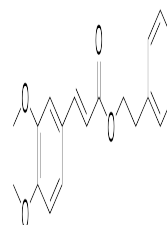
Chemical structure of Phenethyl Dimethyl...
