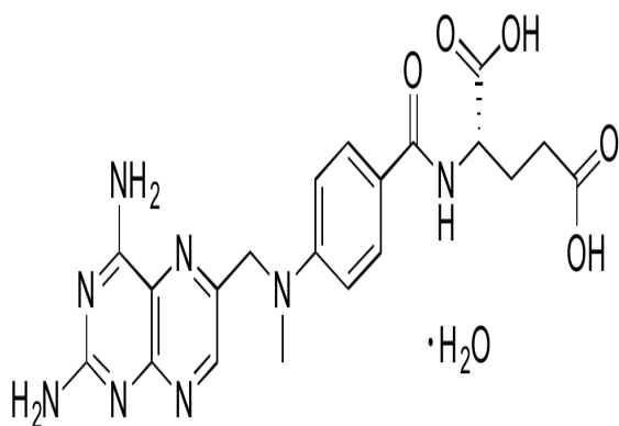
Chemical structure of Methotrexate Hydrate
