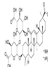
Chemical structure of Glycyrrhizic Acid ...
