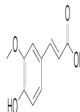
Chemical structure of Ferulic Acid
