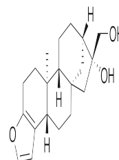
Chemical structure of Cafestol
