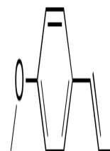
Chemical structure of trans- Anethole
