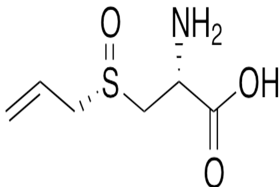
Chemical structure of L-(+)-Alliin
